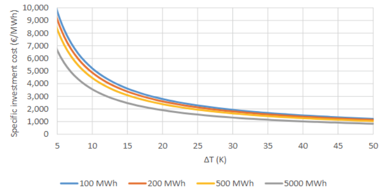
ATES investment cost as a function of temperature difference (for a fixed storage capacity)
